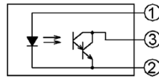
Internal Circuit
