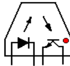
Internal Circuit
